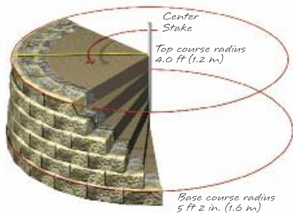
Base Course Radius for an outside curve on a 4 ft tall 6° wall
