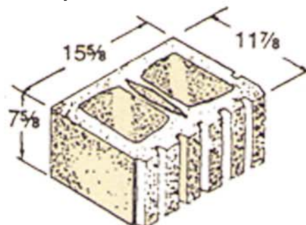
12 x 8 x 16 Hollow Split Fluted
