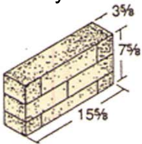
4 x 8 x 16 Hollow Style A*
