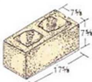
8 x 8 x 18 Hollow
