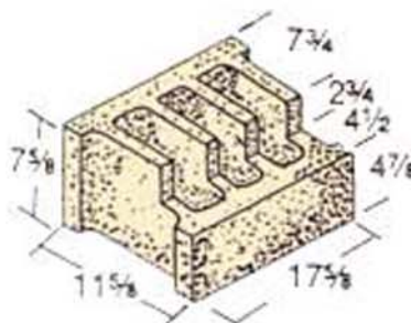
12 x 8 x 18 Header*
