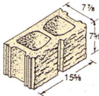
8 x 8 x 16
