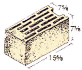
8 x 8 x 16 Hollow Corner
