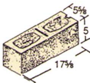
6 x 5 x 18 Hollow
