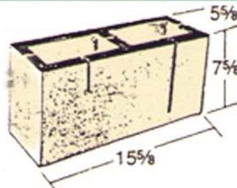
6 x 8 x 16 Type A
