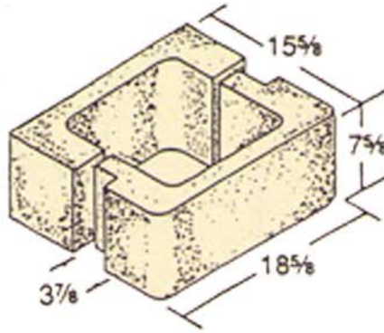
16 x 8 x 19 Pilaster Flush Wall Construction*
