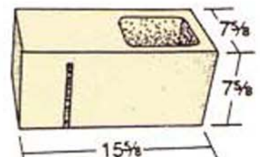
8 x 8 x 16 Vertical Reinforcement Soundblox Right
