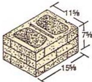
12 x 8 x 16 Hollow Style B
