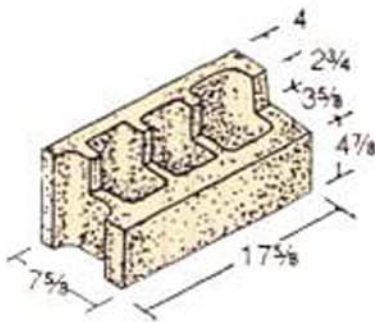
8 x 8 x 18 Header*
