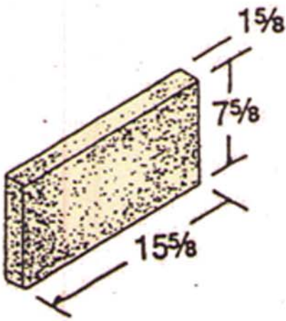
2 X 8 16 Solid
