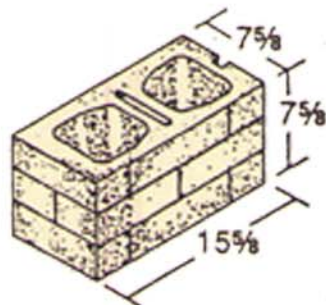
8 x 8 x 16 Hollow Style B
