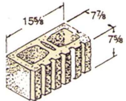
8 x 8 x 16 Hollow Split Fluted
