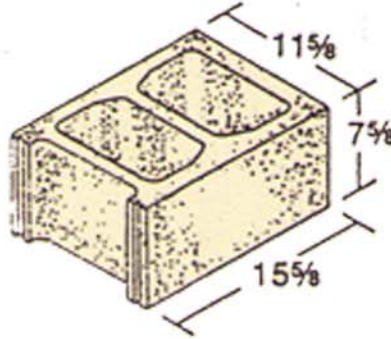
12 x 8 x 16 Hollow
