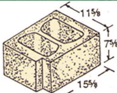
12 x 8 x 16 Hollow With 1 3/4" x 1 3/4" Notch
