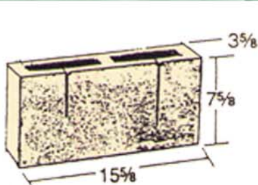
4 x 8 x 16 Type A
