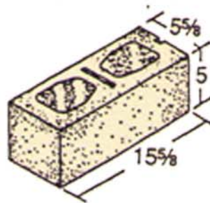
6 x 5 x 16 Hollow
