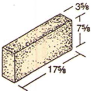
4 x 8 x 18 Solid
