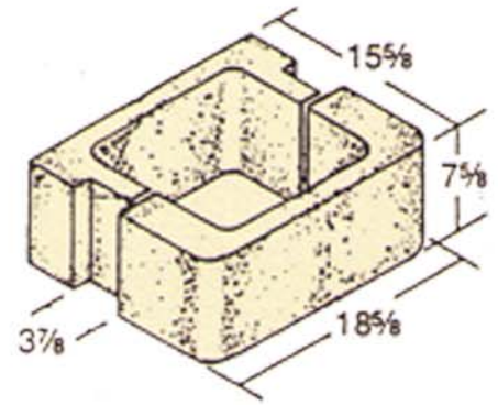
16 x 8 x 19 Pilaster Finish Wall Construction*
