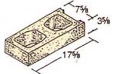
8 x 4 x 18 Hollow
