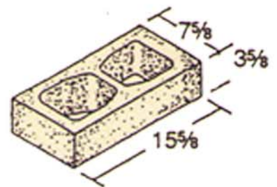
8 x 4 x 16 Hollow
