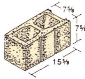
8 x 8 x 16 Double Score
