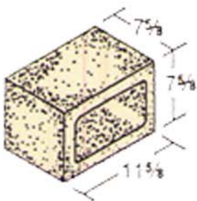
8 x 8 x 12 Solar
