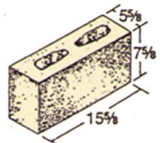
6 x 8 x 16 (75% Solid)
