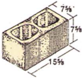
8 x 8 x 16 Single Score
