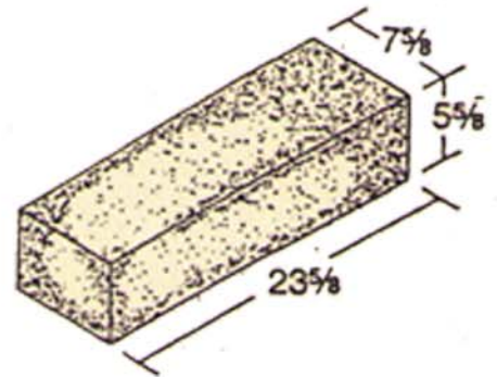
6 x 8 x 24 Solid*
