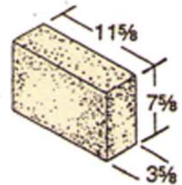
4 x 8 x 12 Hollow
