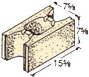
8 x 8 x 16 Open End
