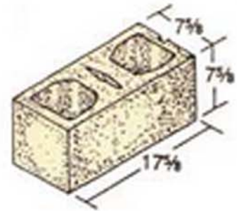
8 x 8 x 18 Hollow 4 Hour Fire Rated*
