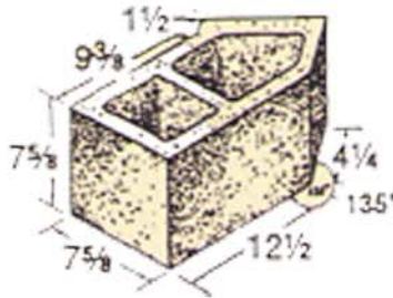
8" Angle Block with Leg*
