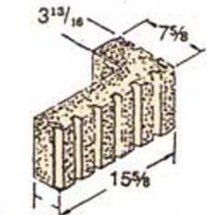
4" L Corner Split Fluted
