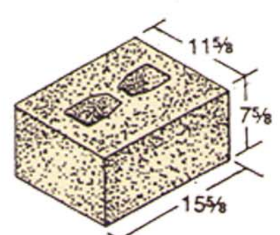
12 x 8 x 16 (75% Solid)
