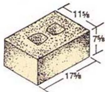
12 x 8 x 18 (75% Solid)
