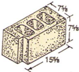
8 X 8 X 16 (75% Solid) With 1 3/4" x 1 3/4" Notch
