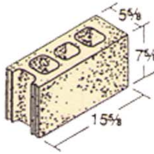
6 x 8 x 16 Female*
