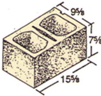
10x 8 x 16 Hollow
