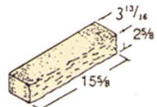
4 X 3 X 16
