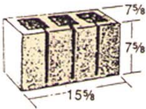
8 x 8 x 16 Type BB
