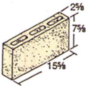
3 x 8 x 16 Hollow
