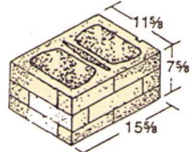
12 x 8 x 16 Hollow Style A
