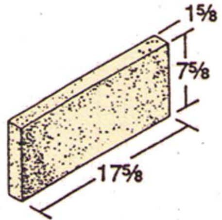
2 X 8 18 Solid
