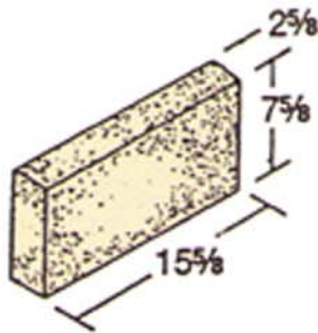
3 x 8 x 16 Solid
