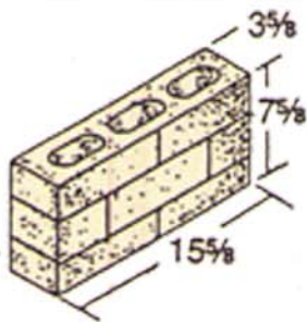
4 x 8 x 16 Hollow Style A*
