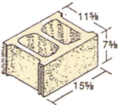
12 x 8 x 16 Hollow
