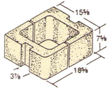
16 x 8 x 19 Pilaster Flush Wall Construction*
