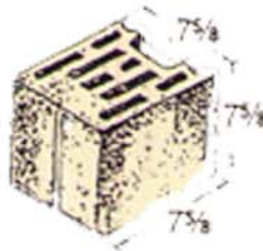
8 x 8 x 8 Hollow With Sash
