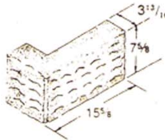
4" L Corner
