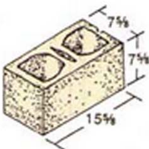
8 x 8 x 16 Hollow 4 Hour Fire Rated*
