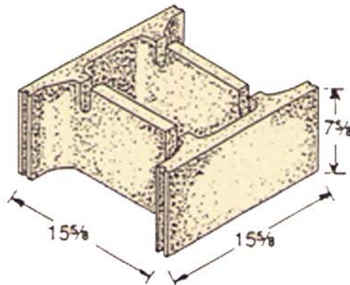
16 x 8 x 16 Open End
