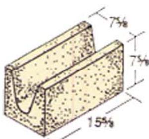
8 X 8 X 16 Beam Lintel
