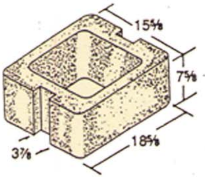
16x 8 x 19 Slot Pilaster Flush Wall Construction*
