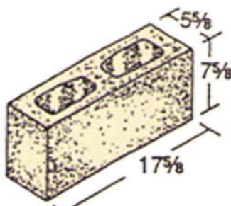
6 x 8 x 18 Hollow
