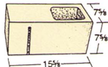
8 x 8 x 16 Vertical Reinforcement Soundblox Right
