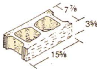
8 x 4 x 16
