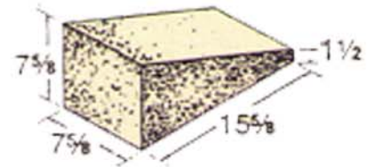
8" Solid Gable Block
