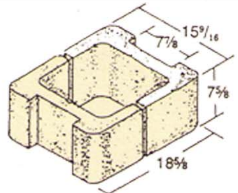
16 x 8 x 19 Pilaster Center Wall Construction*
