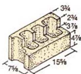
8 x 8 x 16 Header
