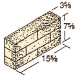
4 x 8 x 16 Solid Style A*
