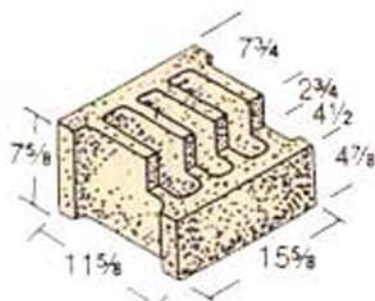
12 x 8 x 16 Header*
