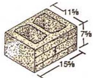
12 x 8 x 16 Hollow Style B
