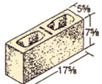
6 x 8 x 18 Hollow
