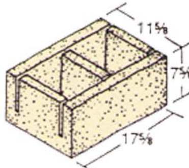
12 x 8 x 18 Bond Beam with Knockouts*
