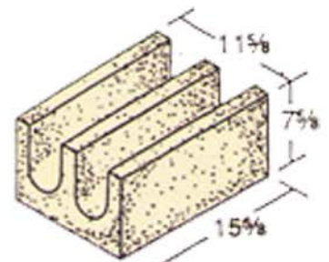
12 x 8 x 16 Beam Lintel
