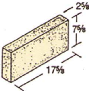
3 x 8 x 18 Solid
