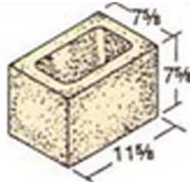
8 x 8 x 12 Hollow
