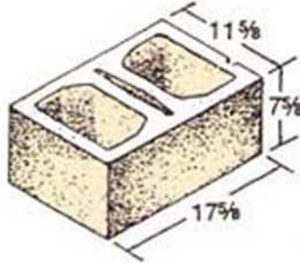
12 x 8 x 18 Hollow
