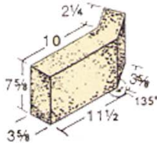
4" Solid Angle Block with Leg*
