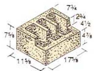
12 x 8 x 18 Header*
