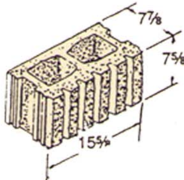
8 x 8 x 16 Hollow Split Fluted
