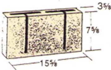
4 x 8 x 16 Type B
