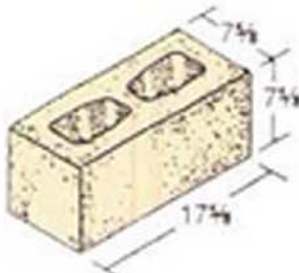
8 x 8 x 18 (75% Solid)
