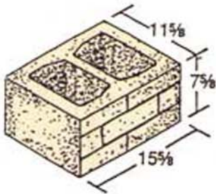
12 x 8 x 16 Hollow Style A
