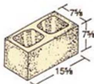
8 x 8 x 16 Hollow 4 Hour Fire Rated*
