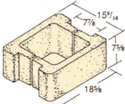
16 x 8 x 19 Pilaster Center Wall Construction*
