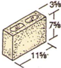
4 x 8 x 12 Hollow*
