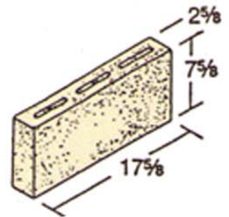
3 x 8 x 18 Hollow
