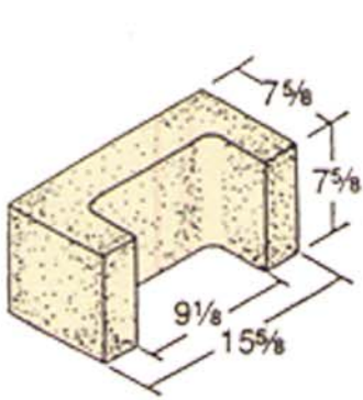
8 x 8 x 16 Chimney Block
