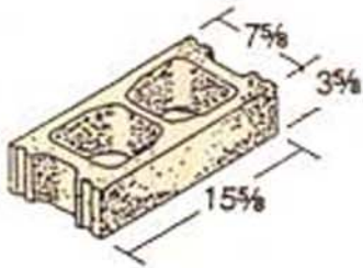
8 x 4 x 16 Hollow
