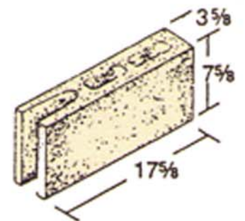
4 x 8 x 18 Hollow w/Open End
