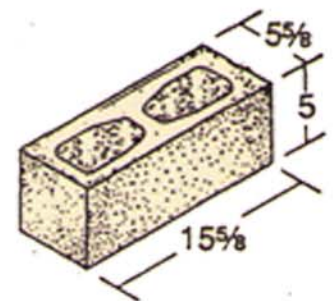
6 x 5 x 16 Hollow
