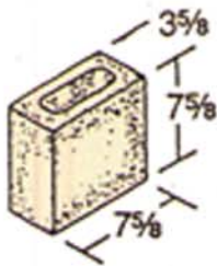
4 x 8 x 4 Hollow
