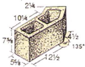
6" Angle Block* with Leg*
