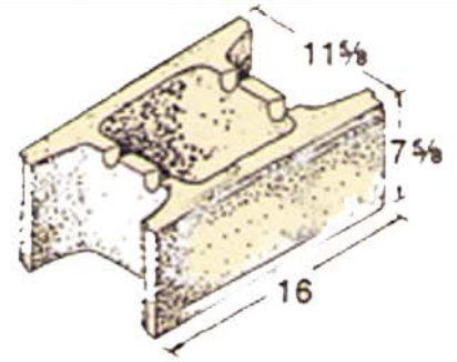
12 x 8 x 16 Open End
