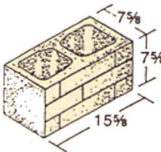
8 x 8 x 16 Hollow Style B
