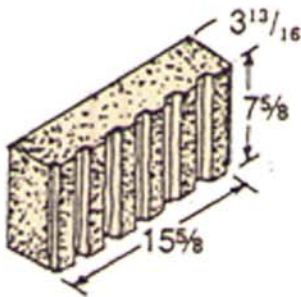
4 X 8 X 16 Solid Split Fluted
