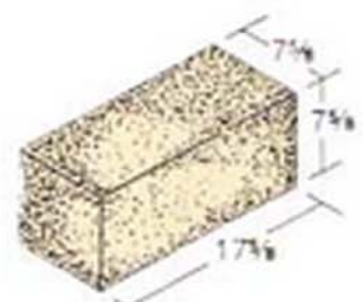
8 x 8 x 18 (75% Solid) *
