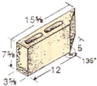
4" Angle Block*
