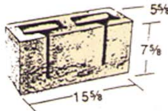
6 x 8 x 16 Type R
