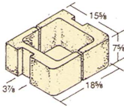
16 x 8 x 19 Pilaster Finish Wall Construction*
