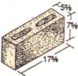
6 x 8 x 18 (75% Solid)
