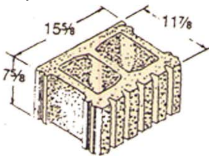
12 X 8 X 16 Hollow Split Fluted
