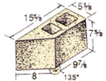
6" Angle Block*
