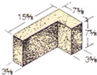
4" L Solid*
