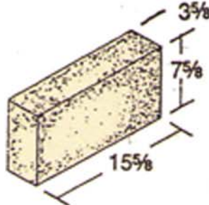
4 x 8 x 16 Solid
