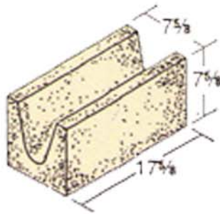
8 x 8 x 18 Beam Lintel*
