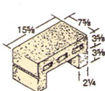
4 Pallet Block (4 x 16 Hollow + 2 Brick)*
