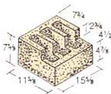
12 x 8 x 16 Header*
