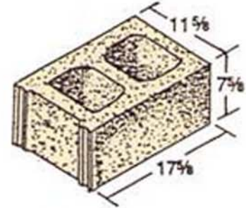
12 x 8 x 18 Hollow
