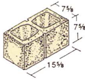
8 x 8 x 16 Single Score (Both Sides)
