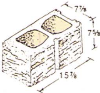
8 x 8 x 16 Corner Return
