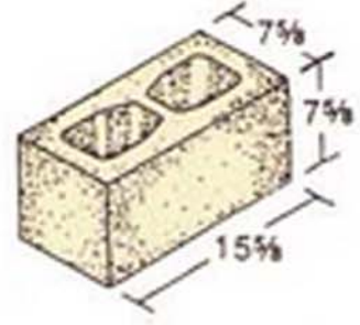
8 x 8 x 16 (75% Solid)
