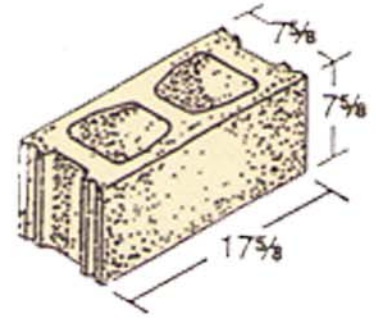
8 x 8 x 18 Female
