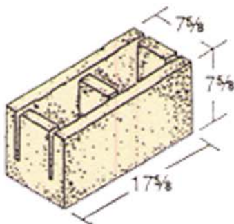
8 x 8 x 18 Bond Beam with Knockouts*
