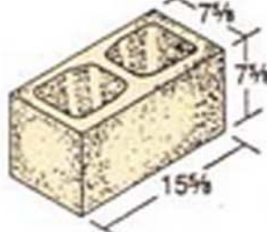
8 x 8 x 16 Hollow
