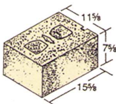
12 x 8 x 16 (75% Solid)
