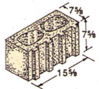
8 x 8 x 16 Molded Fluted*
