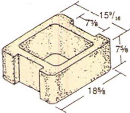
16 x 8 x 19 Pilaster Center Wall Construction*
