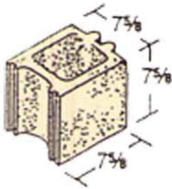
8" Half Male*
