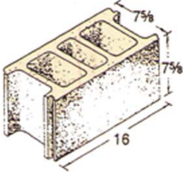
8 x 8 x 16 Slot*
