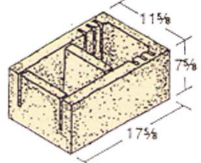
12 x 8 x 18 Bond Beam with Knockouts*
