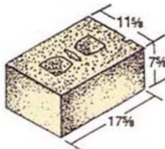
12 x 8 x 18 (75% Solid)
