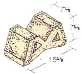
8 X 8 X 16 Double A Screen
