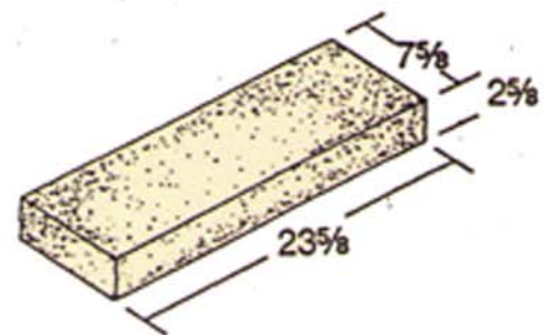
3 x 8 x 24 Solid*
