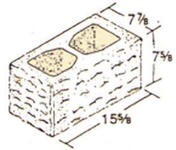
8 x 8 x 16 Corner Return
