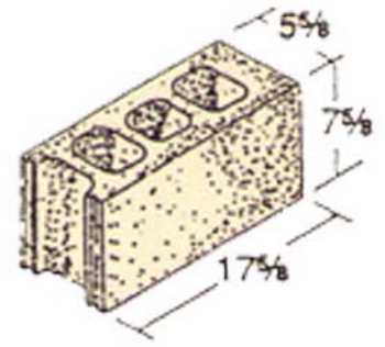
6 x 8 x 18 Female*
