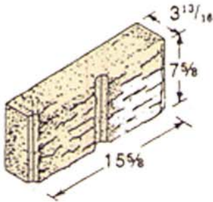
4 x 8 x 16 Solid
