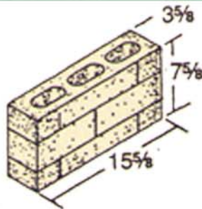
4 x 8 x 16 Hollow Style B*
