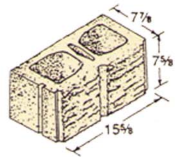
8 x 8 x 16
