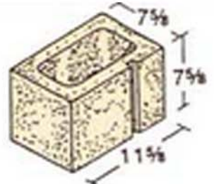
8 x 8 x 12 Hollow
