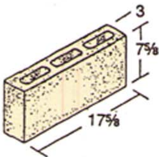
3 x 8 x 18 Hollow* Full 3". not 2 5/8"
