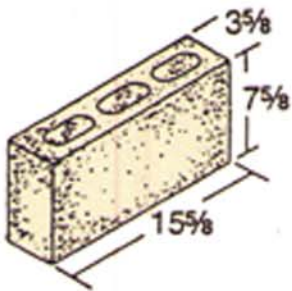
4 x 8 x 16 Hollow
