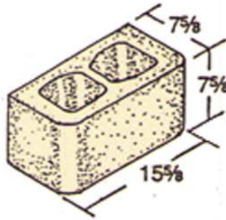
Double Bullnose on same side*
