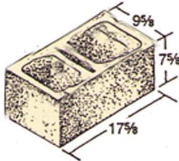
10 x 8 x 18 Hollow
