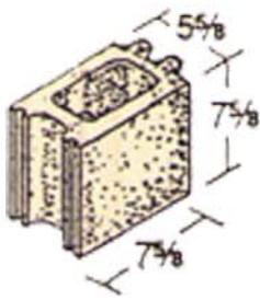
6" Half Male*
