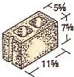
6 x 8 x 12 Hollow*
