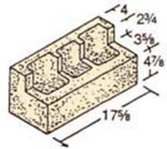
8 x 8 x 16 Header*
