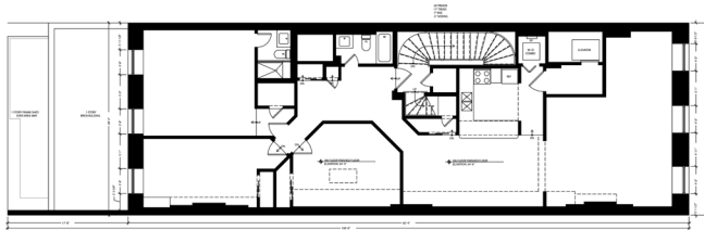
5th Floor
